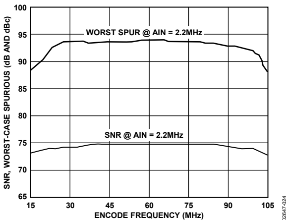
Figure 18. SNR, Worst-Case Spurious vs. Encode @ 2.2 MHz
