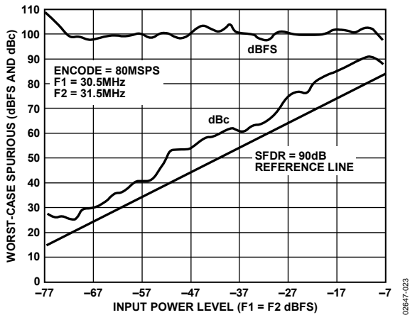
Figure 17. Two-Tone SFDR @ 30.5 MHz and 31.5 MHz
